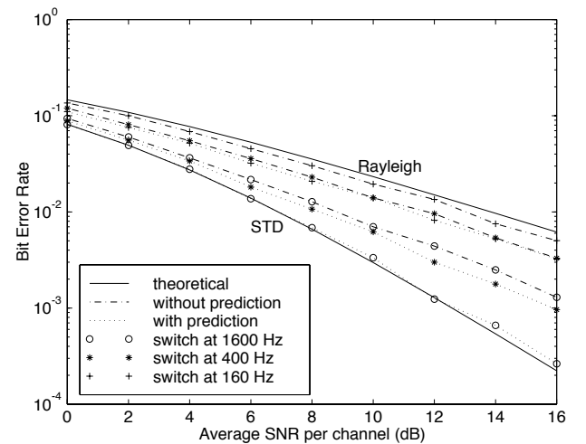
Figure 3. BER performance of STD over flat Rayleigh fading channel with and without prediction for various antenna switching rates. ( f_{dm} = 200 Hz, 9-oscillator Jakes model).
