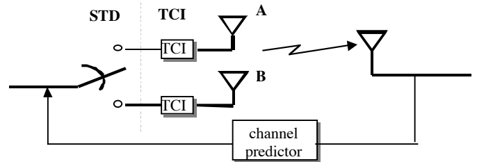
Figure 6 Driving configuration of STD + TCI scheme.
