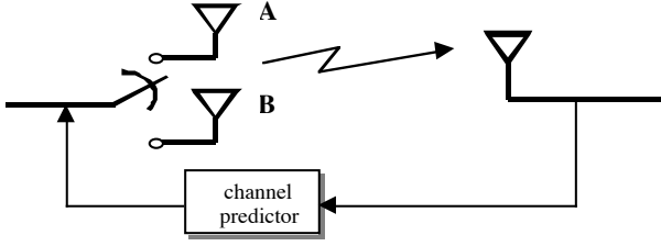
Figure 1. Operation of STD for two transmitter antennas
