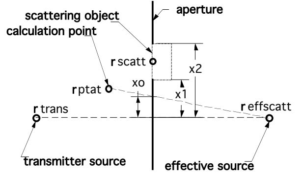
Figure 1. The parameters used to calculate the amplitude from one reflecting object, shown as a dotted rectangle. Also shown is the aperture chosen. The origin is arbitrary since only differences between the vectors are used.
