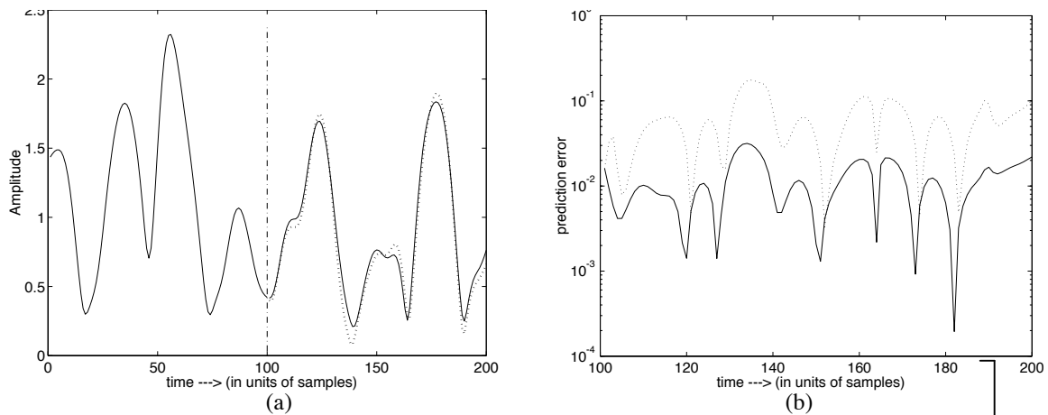
Figure 1. Testing long range prediction algorithm for measured data. (a) Prediction 3 steps ahead (0.9 ms). First half: the actual fading channel envelope (solid) is observed. Second half: the actual future (solid) and predicted (dotted) fading channel envelopes. (b) Prediction error comparison for predicting 1 step (solid) and 3 steps (dotted) ahead.
