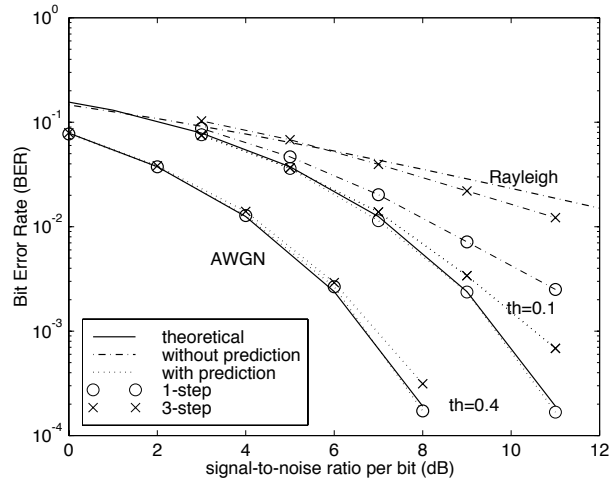
Figure 2. Bit Error Rate vs. Average SNR: Theoretical: TCI at each threshold (th) level for Rayleigh fading channel. Without Prediction: TCI using delayed feedback for measured data (th=0.1, 1 and 3 step delay); no adaptation (Rayleigh fading channel). With Prediction: joint long range prediction (1 and 3 steps, th=0.1 and 0.4) and TCI for measured data.
