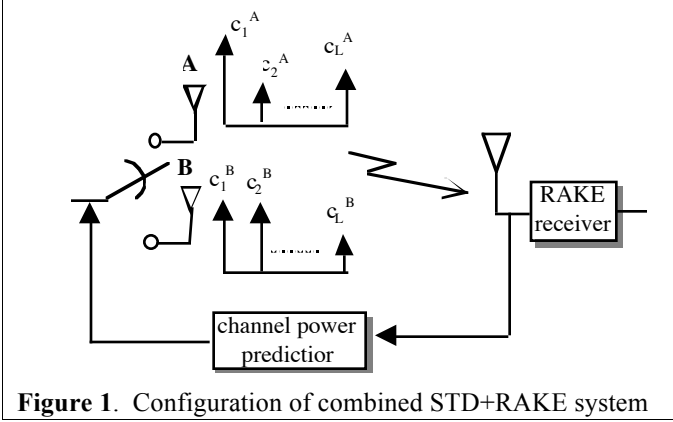
Figure 1. Configuration of combined STD+RAKE system
