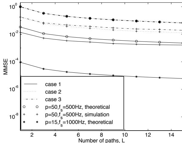
Figure 2. Prediction MSE of total multipath channel power. Prediction range \tau=2\text{ms} .
