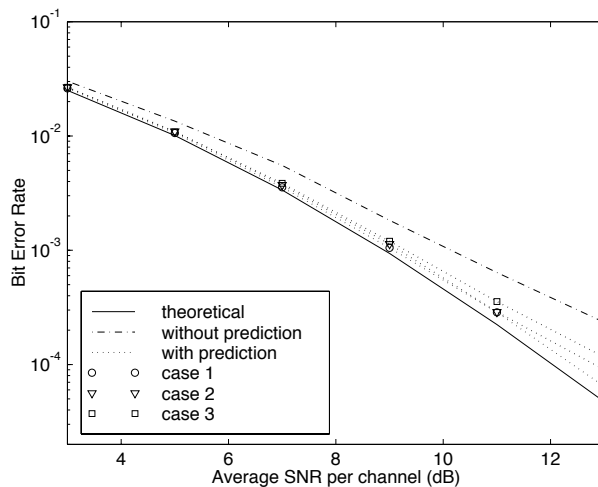
Figure 5. BER performance comparison of STD+RAKE (switching frequency 1.6KHz, L=2 ) without prediction and for three power prediction methods.
