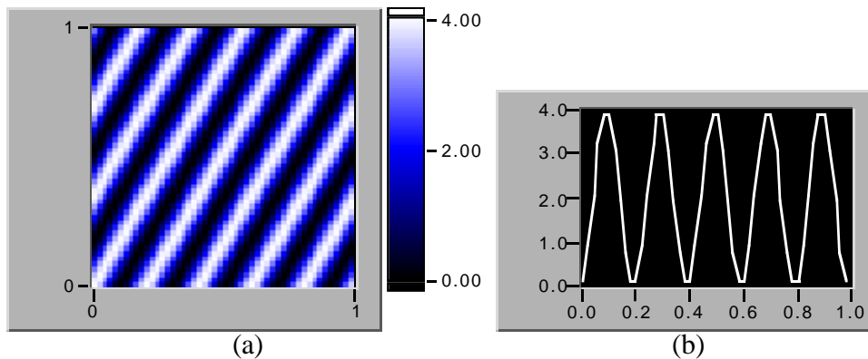
Figure 1. (a) The interference pattern for two plane wave sources one incident from the left and the other from the lower right 60° below horizontal. The frequency is 1 GHz and the image 1 m on a side. (b) A horizontal cut through the image half way up the image in (a).
