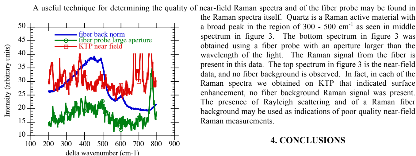
Figure 3. Raman scattering from the quartz fiber is observed in a large aperture probe, but not in the near-field spectrum indicating a surface enhancement.
